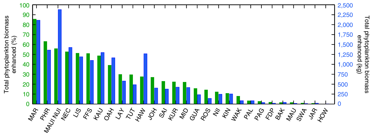
Figure 5 | Total phytoplankton biomass enhanced near Pacific island- and atoll-reef ecosystems. Bars represent the total increase in long-term phytoplankton biomass at each location over offshore, oceanic phytoplankton biomass. Values are shown in percentage (green bars; left y-axis) and kg (blue bars; right y-axis), oriented in decreasing percent biomass from left to right. All locations had significant linear fits ( P < 0.05 ).
