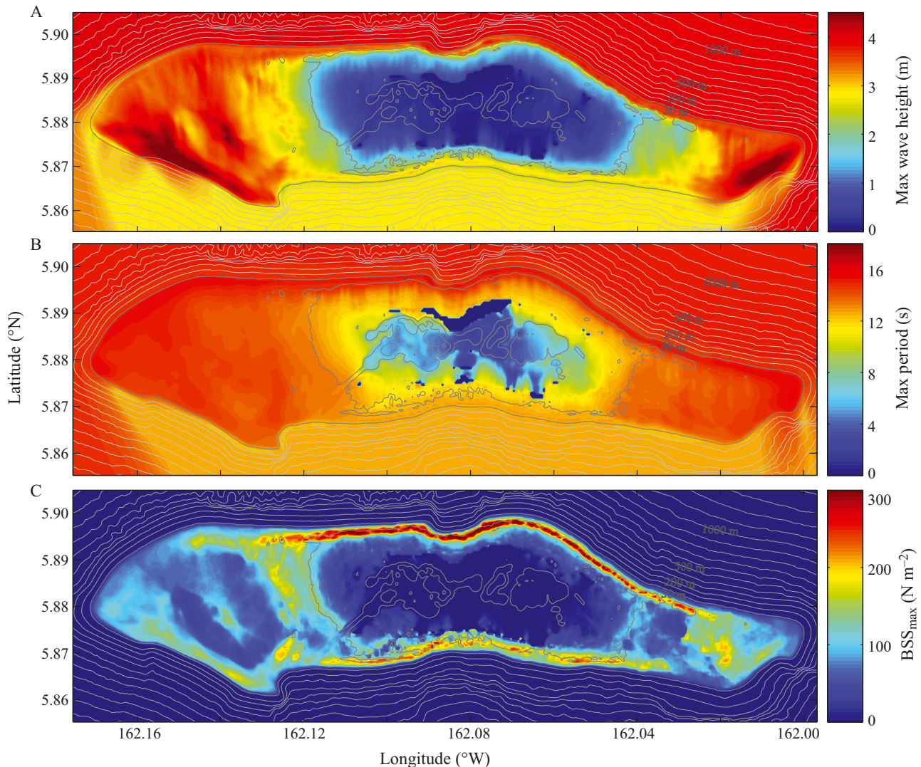
Fig. 4. Hydrodynamic wave model results representing the maximum values of (A) significant wave height, (B) wave period, and (C) bed shear stress ( BSS_{max} ) at Palmyra Atoll. Results represent the maximum of each grid cell from the combined hydrodynamic model runs for each swell regime (i.e. northwest swell, northeast trade wind swell, and south swell) at Palmyra Atoll (see Fig. 1)
